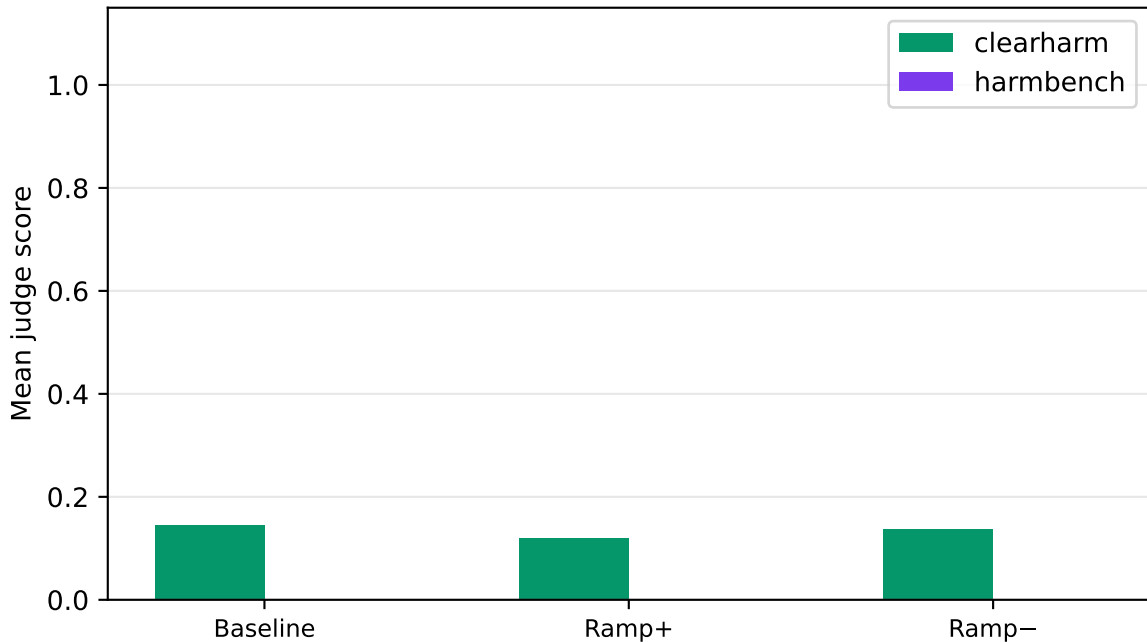
llama-3.1-8b | safety | k=0.25 — by source
