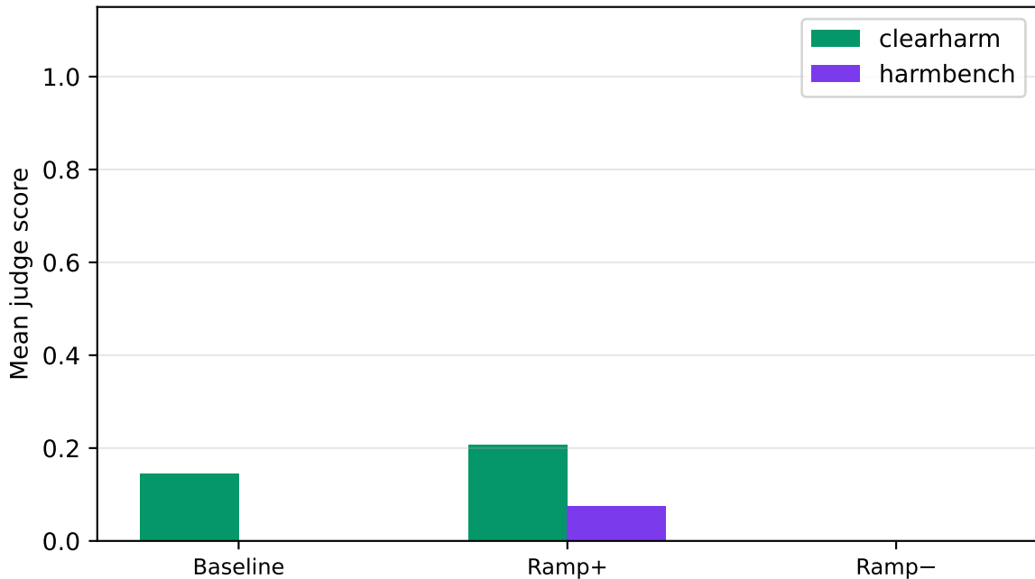
llama-3.1-8b | safety | k=2.00 — by source
