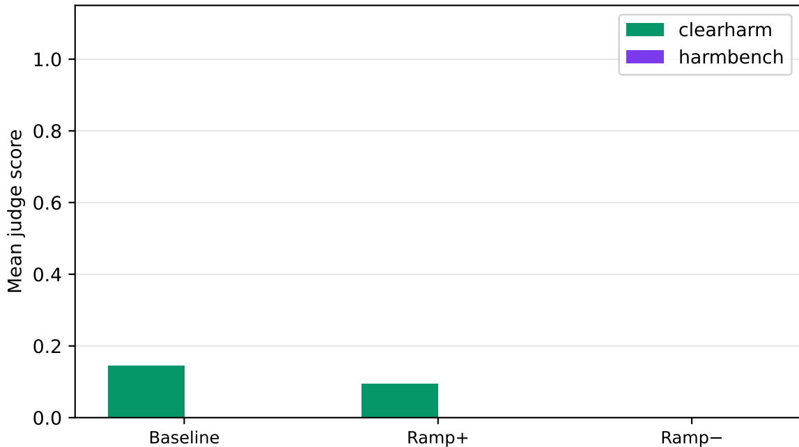
llama-3.1-8b | safety | k=3.00 — by source
