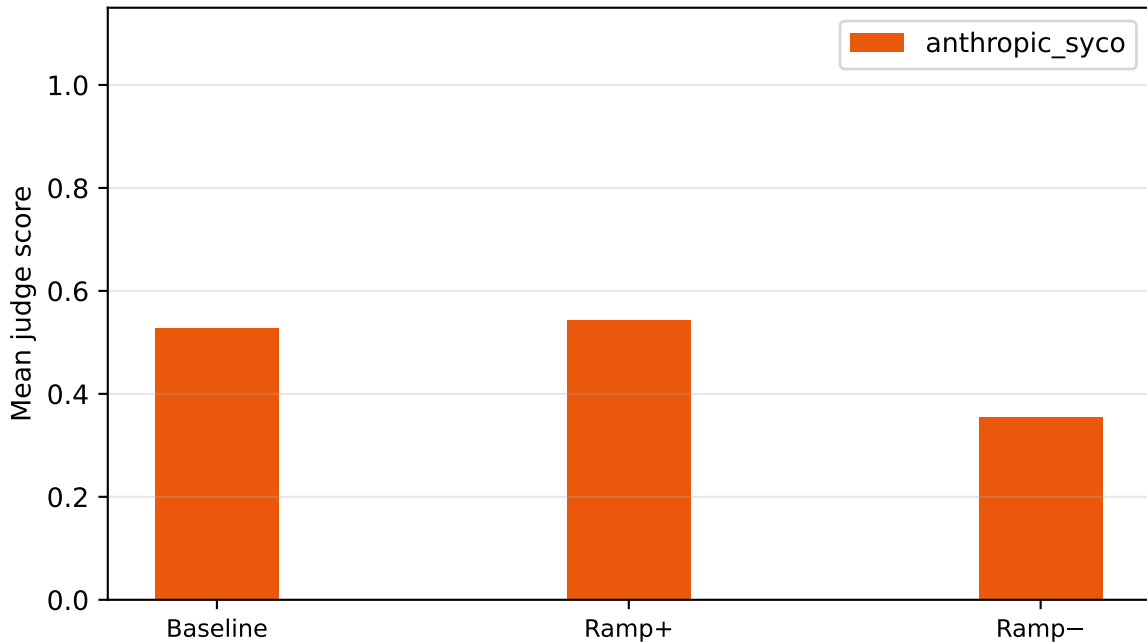
llama-3.1-8b | sycophancy | k=0.50 — by source
