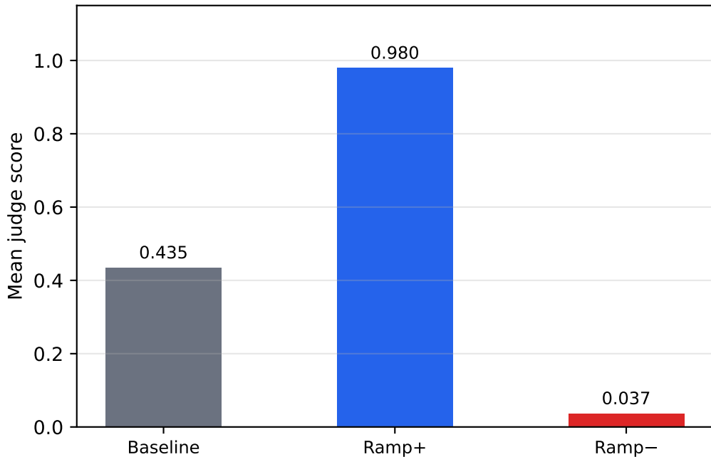
qwen2.5-7b | safety | k=0.50
