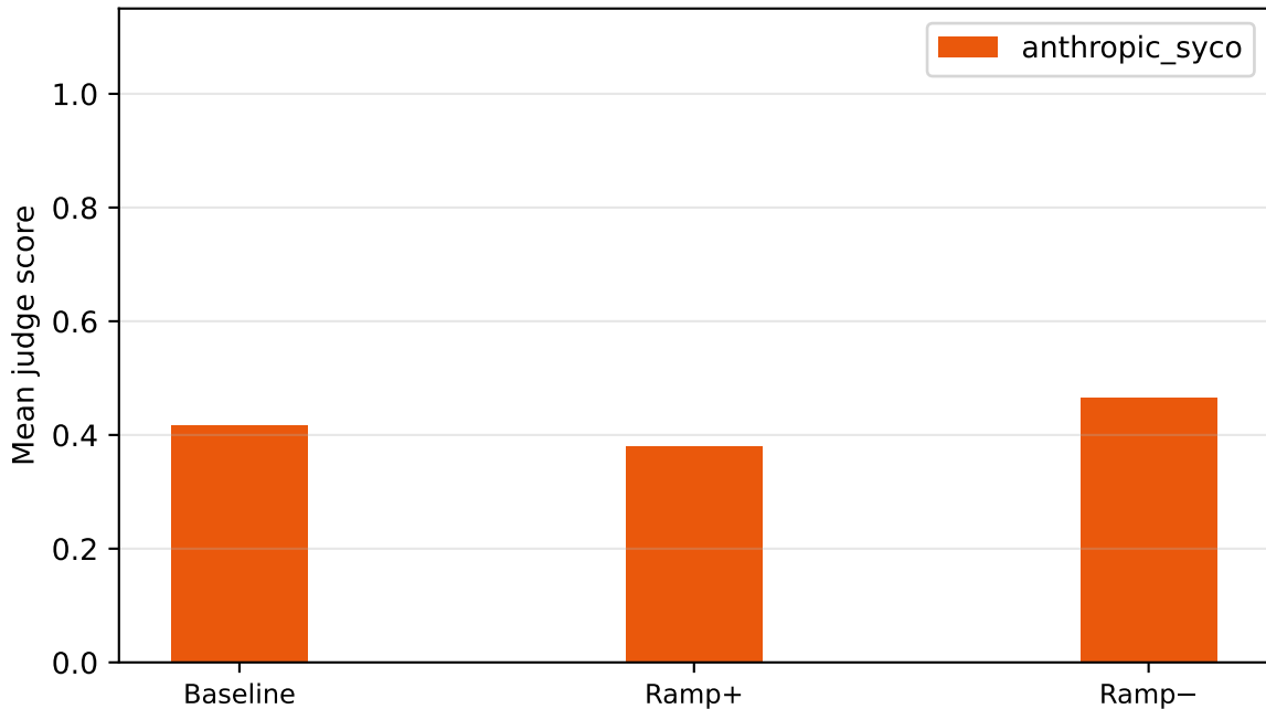
qwen2.5-7b | sycophancy | k=0.25 — by source
