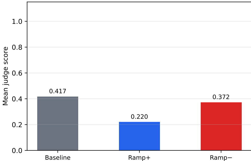
qwen2.5-7b | sycophancy | k=0.50
