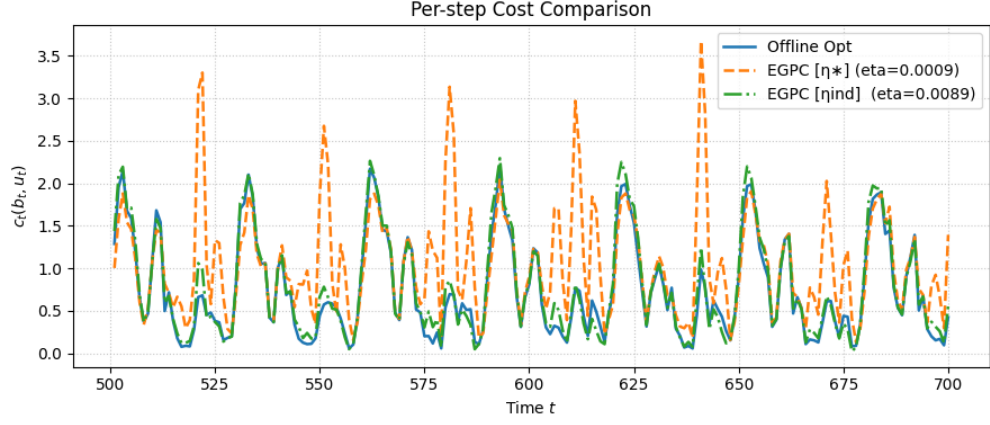
Figure 8: Instantaneous costs for EGPC (two step sizes) versus the offline-optimal policy for t \in [500, 700] , with \kappa = 0.1 . This figure demonstrates how the cost curves compress as the algorithm approaches stable behavior.
