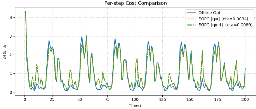
Figure 19: Instantaneous costs for EGPC (two step sizes) versus the offline-optimal policy for t \in [0, 200] , with \kappa = 0.4 . This interval shows the initial fluctuation in costs as the controller adapts.
