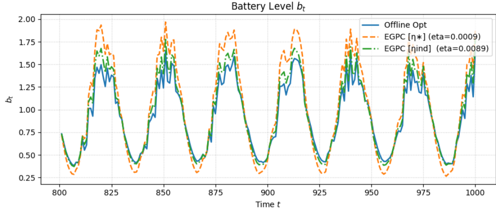
Figure 5: State levels for EGPC (two step sizes) versus the offline-optimal policy for t \in [800, 1000] , with \kappa = 0.1 . By this stage, the controller has largely stabilized and the trajectories cluster tightly.
