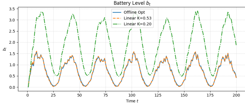
Figure 14: State levels for the linear controllers ( K = 0.53 and K = 0.20 ) versus the offline-optimal policy for t \in [0, 200] , with \kappa = 0.4 . The linear controllers produce repetitive, time-invariant behavior.
