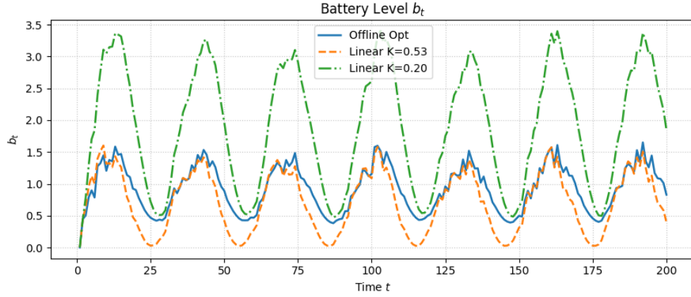
Figure 2: State levels for the linear controllers ( K = 0.53 and K = 0.20 ) versus the offline-optimal policy for t \in [0, 200] , with \kappa = 0.1 . The linear controllers produce repetitive, time-invariant behavior.
