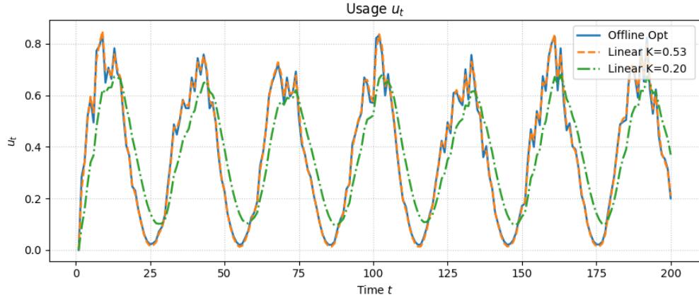
Figure 22: Usage u_t for the linear controllers versus the offline-optimal policy for t \in [0, 200] , with \kappa = 0.4 .
