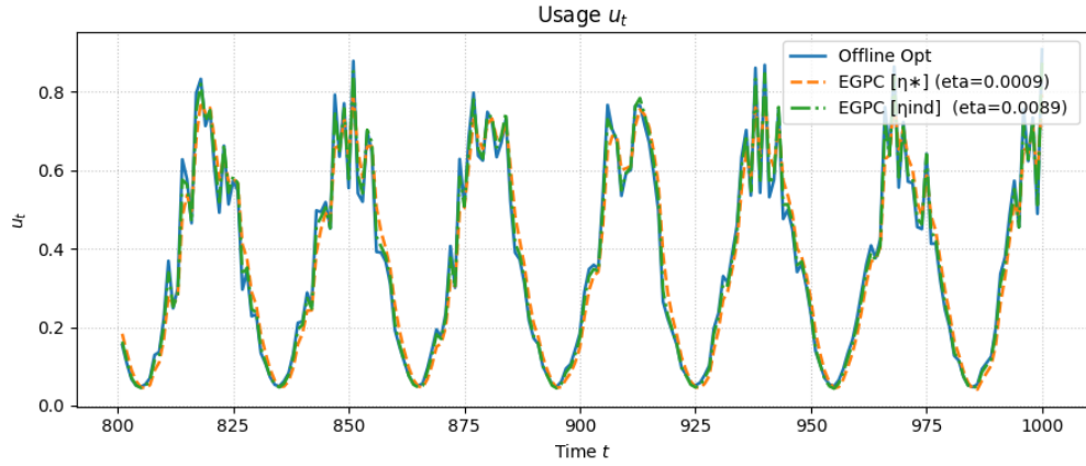
Figure 13: Usage u_t for EGPC (two step sizes) versus the offline-optimal policy for t \in [800, 1000] , with \kappa = 0.1 . This final segment shows the stabilization of usage decisions around the offline-optimal policy.
