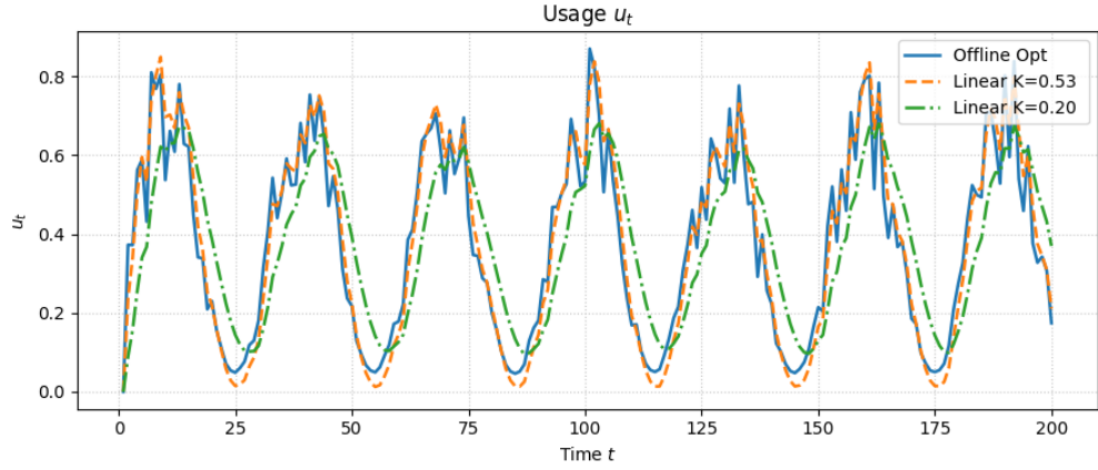
Figure 10: Usage u_t for the linear controllers versus the offline-optimal policy for t \in [0, 200] , with \kappa = 0.1 .
