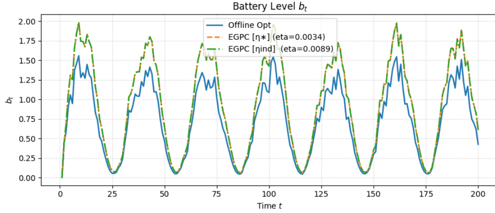
Figure 15: State levels for EGPC (two step sizes) versus the offline-optimal policy for t \in [0, 200] , with \kappa = 0.4 . This interval highlights the initial transient behavior before the controller stabilizes.
