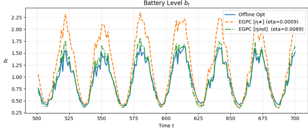
Figure 4: State levels for EGPC (two step sizes) versus the offline-optimal policy for t \in [500, 700] , with \kappa = 0.1 . This mid-horizon window illustrates the slow but consistent convergence trend.
