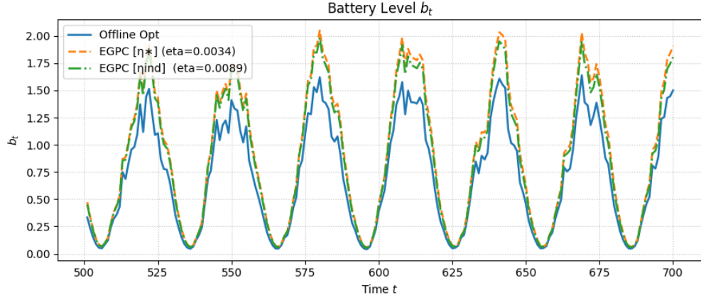
Figure 16: State levels for EGPC (two step sizes) versus the offline-optimal policy for t \in [500, 700] , with \kappa = 0.4 . This mid-horizon window illustrates the slow but consistent convergence trend.
