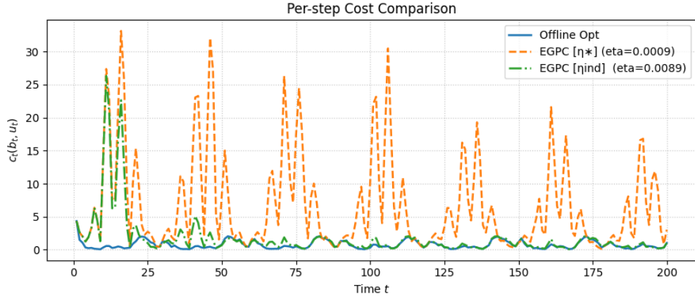
Figure 7: Instantaneous costs for EGPC (two step sizes) versus the offline-optimal policy for t \in [0, 200] , with \kappa = 0.1 . This interval shows the initial fluctuation in costs as the controller adapts.
