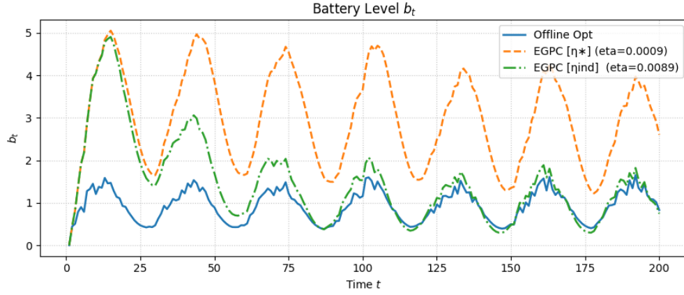
Figure 3: State levels for EGPC (two step sizes) versus the offline-optimal policy for t \in [0, 200] , with \kappa = 0.1 . This interval highlights the initial transient behavior before the controller stabilizes.
