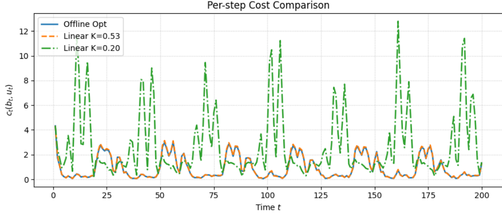
Figure 18: Instantaneous costs for the linear controllers versus the offline-optimal policy for t \in [0, 200] , with \kappa = 0.4 .
