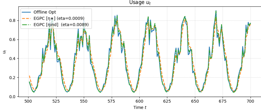
Figure 12: Usage u_t for EGPC (two step sizes) versus the offline-optimal policy for t \in [500, 700] , with \kappa = 0.1 . The mid-horizon behavior shows reduced variability and improved alignment with the benchmark.
