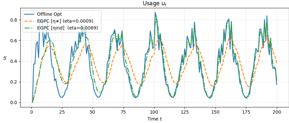
Figure 11: Usage u_t for EGPC (two step sizes) versus the offline-optimal policy for t \in [0, 200] , with \kappa = 0.1 . This interval captures the initial adaptation of the usage decisions.
