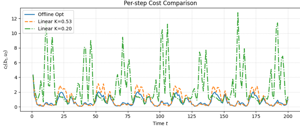
Figure 6: Instantaneous costs for the linear controllers versus the offline-optimal policy for t \in [0, 200] , with \kappa = 0.1 .
