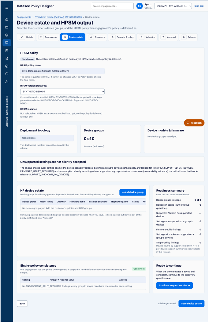
After: “Device estate and HPSM output”; full-width “HPSM policy” card (Not chosen + reason, read-only HPSM policy name, version, instance sentence); the other three cards three across.
