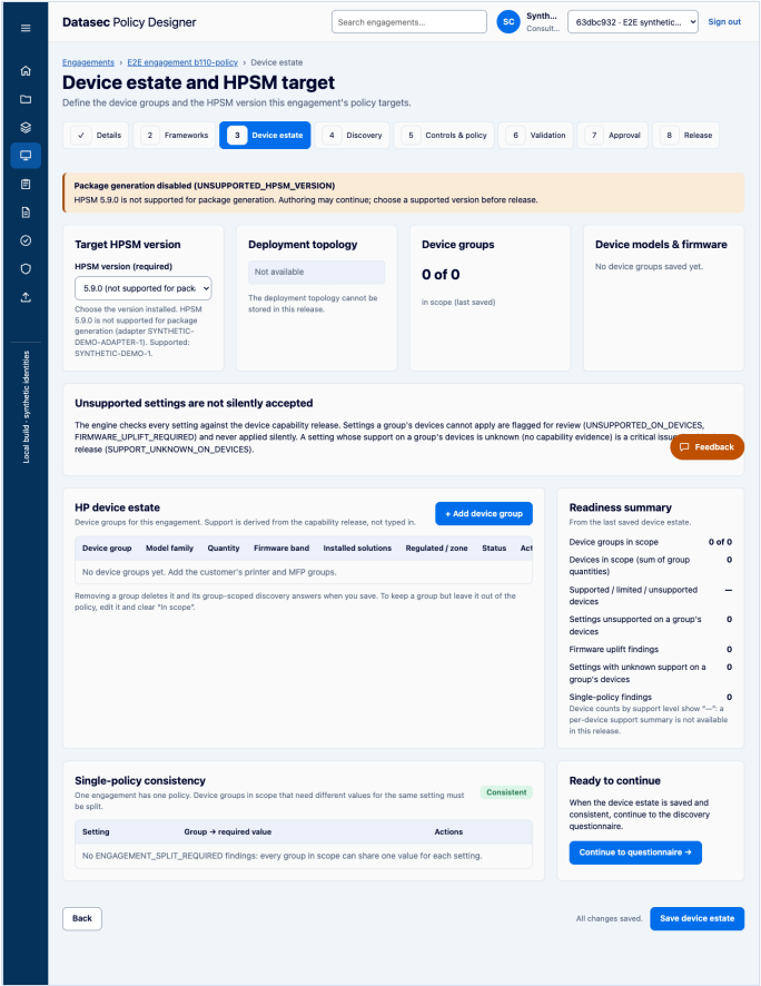
Before: “Device estate and HPSM target”, four cards across, version picker in the first.
