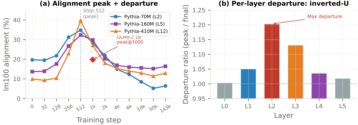
Figure 5. The shortcut-to-full-rank transition. (a) lm_{100} alignment peaks at step 512 across all Pythia sizes, then declines. OLMo-2 1B peaks at step 1,000 (diamond). (b) Per-layer departure ratio follows an inverted-U: middle layers depart most.
