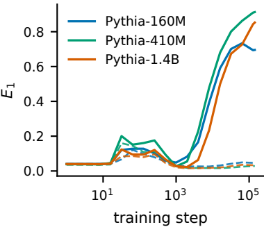
(a) raw (solid), residual (dashed)
