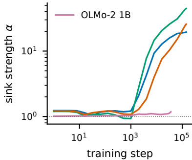
(b) sink strength
