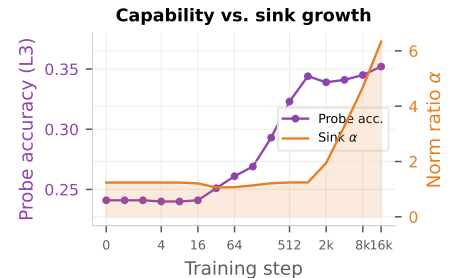
Figure 7. Capability grows monotonically; sink follows a different trajectory. De-sink \Delta < 0.015 throughout.
