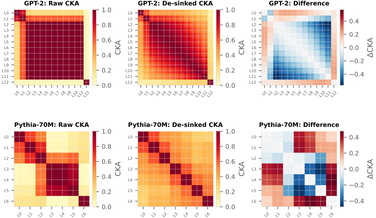
Figure 4. CKA heatmaps. Top: GPT-2. Raw CKA shows L2-L11 as virtually identical ( \approx 1.0 ); de-sinked CKA reveals a rich gradient structure (max |\Delta| = 0.569 ). Bottom: Pythia-70M.
