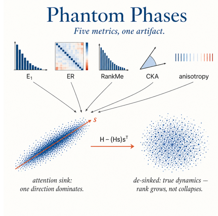
Figure 1. Five metrics, one artifact. Five spectral metrics commonly used to study transformer training— E_1 , effective rank, RankMe, CKA, and anisotropy—all track the same underlying signal: the attention sink, an input-invariant high-variance direction \mathbf{s} that emerges during training. Removing \mathbf{s} via the rank-1 projection \mathbf{H} - (\mathbf{H}\mathbf{s})\mathbf{s}^\top eliminates phantom phase transitions and reveals the true training dynamics: rank grows , not collapses.
