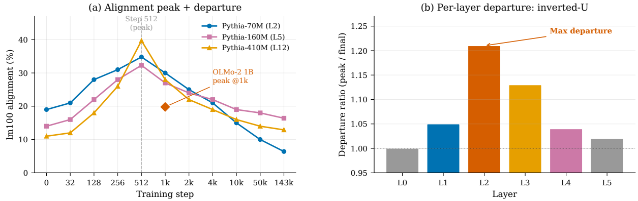
Figure 6. The shortcut-to-full-rank transition. (a) lm100 alignment peaks at step 512 across all Pythia sizes, then declines. OLMo-2 1B peaks at step 1,000 (diamond). (b) Per-layer departure ratio follows an inverted-U: middle layers depart most.
