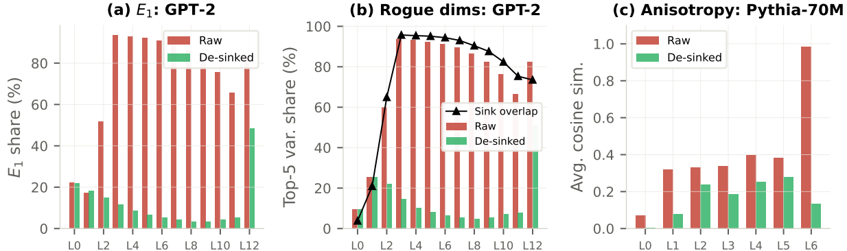
Figure 3. Metric contamination across layers. (a) E_1 in GPT-2: raw 94%, de-sinked 3–12%. (b) Rogue dimensions and sink overlap (>90% at L3–L10). (c) Anisotropy in Pythia-70M: L6 drops from 0.98 to 0.13.
