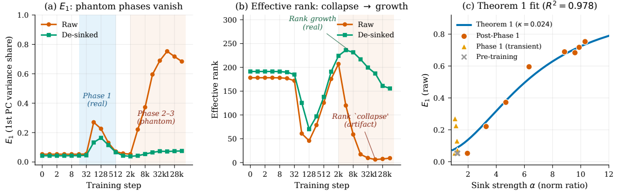
Figure 2. Phantom phases in transformer training (Pythia-70M, L3). (a) Phases 2–3 vanish after de-sinking; only Phase 1 (blue) survives. (b) “Rank collapse” (178 \rightarrow 6.4) reverses to rank growth (191 \rightarrow 236). (c) Theorem 1 predicts contamination with R^2 = 0.978 (one parameter). Phase 1 points (triangles) deviate—content genuinely reorganizes during this period.
