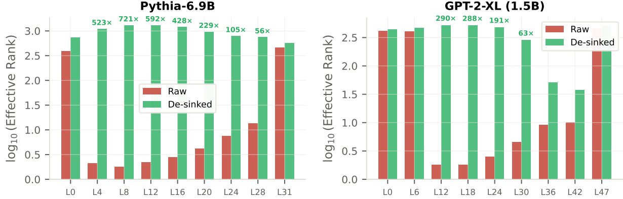
Figure 5. Contamination worsens with scale. ER (log scale) for Pythia-6.9B and GPT-2-XL. Pythia-6.9B L8: 721 \times distortion.
