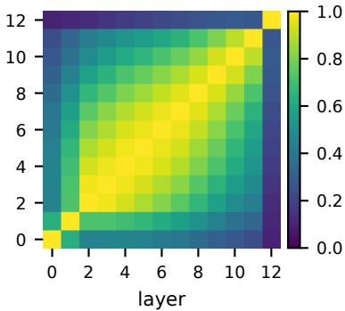
(b) residual CKA
