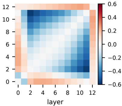
(c) residual minus raw
