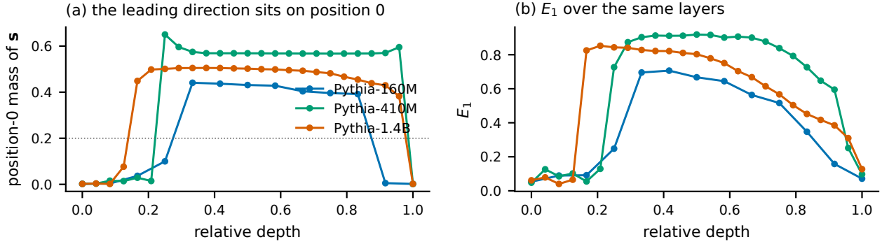
Figure 4: A contiguous band of layers shares one left factor. Final checkpoint, mean over three corpus blocks, depth normalized so the three models overlay. (a) Position-0 mass of the leading direction. Inside the band it is constant to within 0.03; outside it falls below 0.05. This is the hypothesis Proposition 5 needs. (b) E_1 over the same layers, for reference. The two profiles have the same support.
