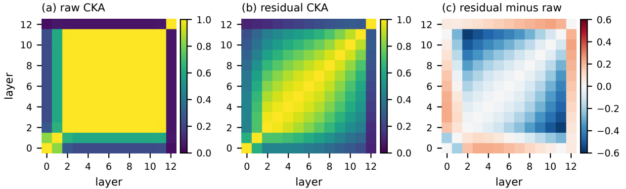
Figure 5: Raw CKA reports one shared direction. GPT-2, 22,819 WikiText-2 tokens. (a) Raw CKA marks L2 through L11 as indistinguishable at \text{CKA} \geq 0.995 . (b) After the projection the same layers show a gradient in depth. (c) The difference. The largest single change is -0.569 between L2 and L11, the pair raw CKA rates most similar.
