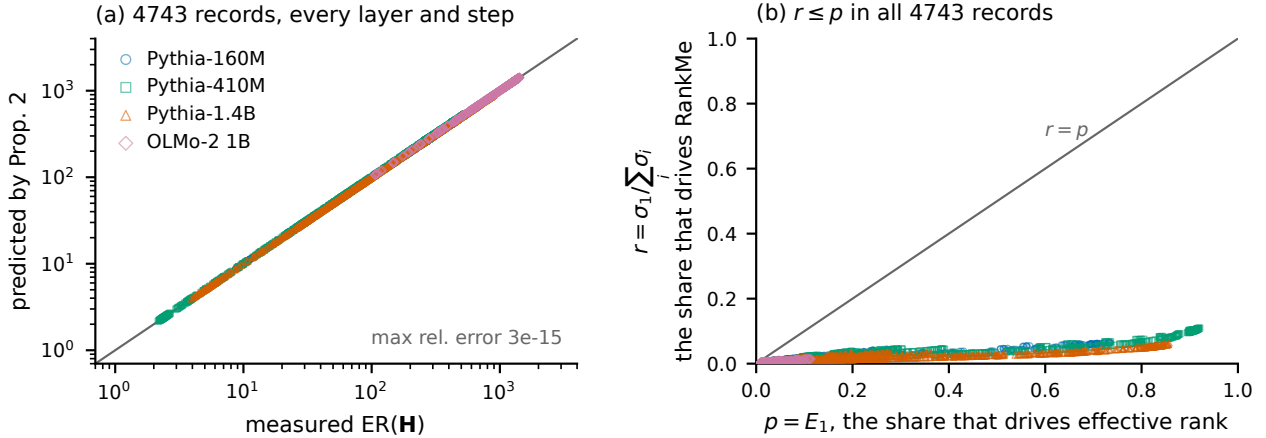
Figure 1: The value of a rank statistic is fixed by one share and the residual. (a) Effective rank predicted by Equation 8 against the measured value, on every record we hold: Pythia at 160M, 410M and 1.4B over 20 checkpoints, OLMo-2 1B over 13, all layers of each, three disjoint corpus blocks, and the 300-record sample-size sweep of Table 10. 4,743 points in total. The largest relative error is 2.9 \times 10^{-15} , at the level of double precision. (b) The two shares. Effective rank is driven by p = E_1 and RankMe by r = \sigma_1 / \sum_i \sigma_i . Lemma 2 forces r \leq p ; the median ratio is 6.2 and the largest is 20.6. Points near p = 1 and r \approx 0.06 are the converged Pythia checkpoints, where the same direction destroys effective rank and barely moves RankMe.
