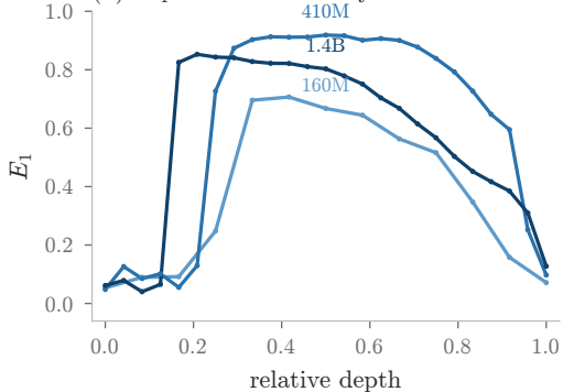
(b) E_1 over the same layers
