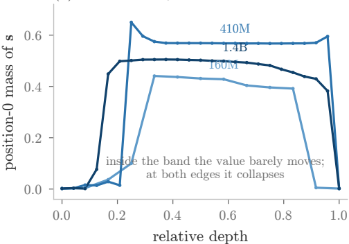
(a) a band of layers shares one left factor
