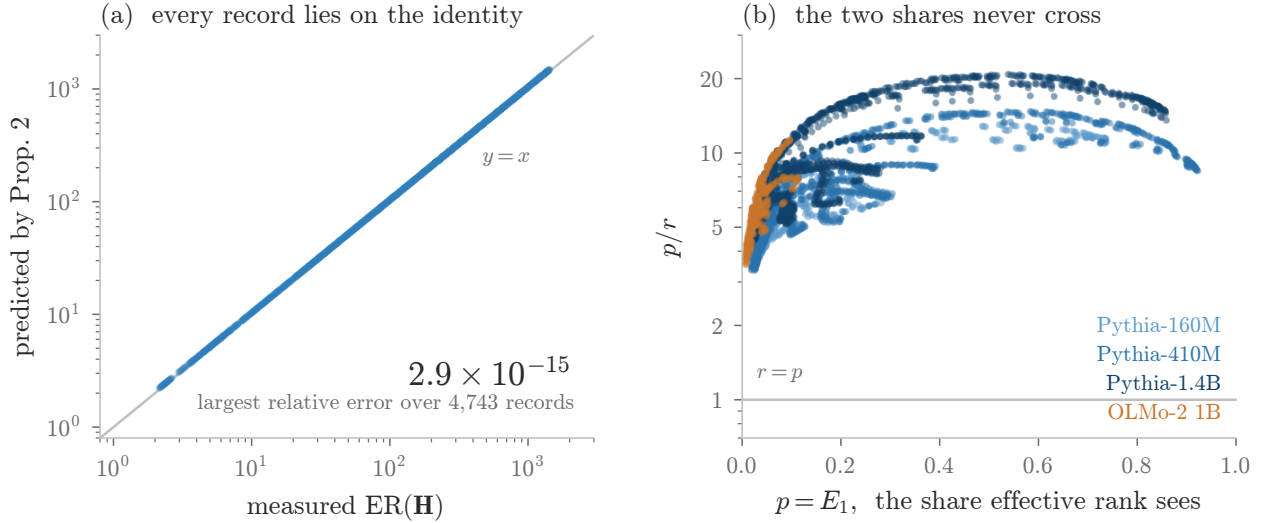
Figure 1: The value of a rank statistic is fixed by one share and the residual. (a) Effective rank predicted by Equation 8 against the measured value, on every record we hold: Pythia at 160M, 410M and 1.4B over 20 checkpoints, OLMo-2 1B over 13, all layers of each, three disjoint corpus blocks, and the 300-record sample-size sweep of Table 8. 4,743 points in total. The largest relative error is 2.9 \times 10^{-15} , at the level of double precision. (b) The ratio of the two shares, p = E_1 for effective rank against r = \sigma_1 / \sum_i \sigma_i for RankMe. Lemma 2 forces r \leq p , so every record sits above p/r = 1 and none crosses; the median is 6.2 and the largest 20.6. The converged Pythia checkpoints on the right carry p near 0.9 against r near 0.06.
