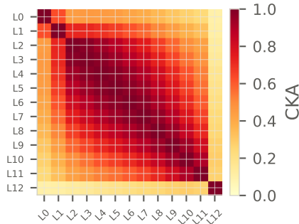
GPT-2: De-sinked CKA
