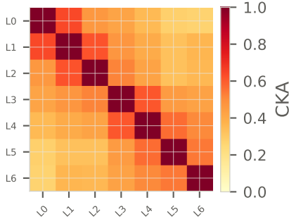
Pythia-70M: De-sinked CKA
