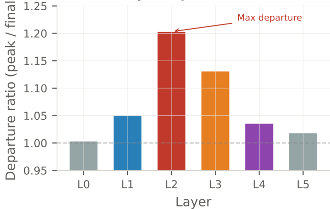
(b) Per-layer departure: inverted-U
