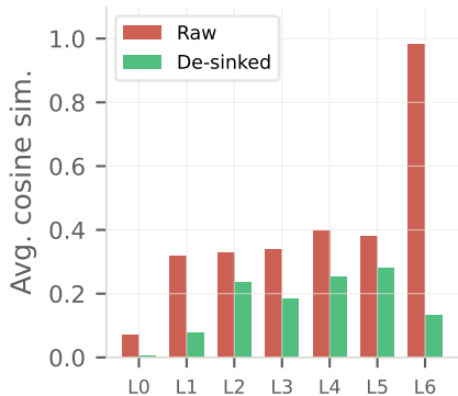
(c) Anisotropy: Pythia-70M
