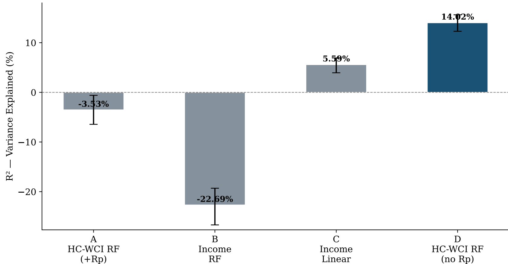
Figure 1: HC-WCI vs Income-Only Baselines (95% Bootstrap CI)
