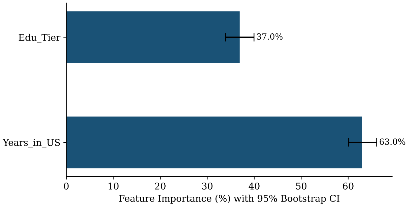
Figure 4: HC-WCI Feature Importance (Model D) Gini Impurity, 200-iteration Bootstrap
