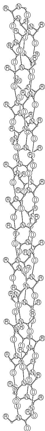
47/13 ALPHA HELIX
