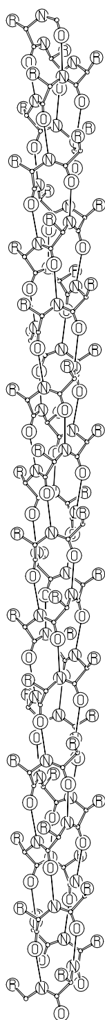
47/13 ALPHA HELIX
