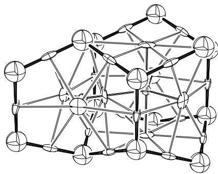
HEXAGONAL DIAMOND
