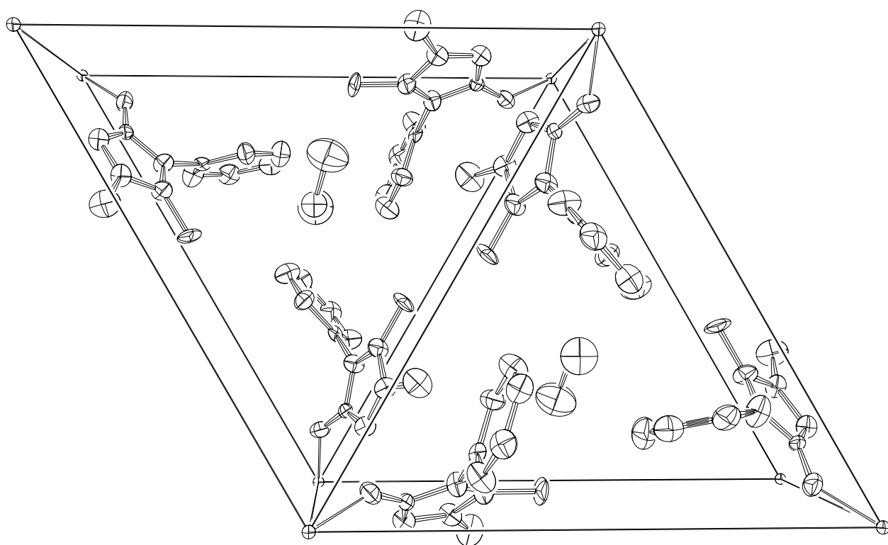
MAGNESIUM HEXAANTIPYRINE PERCHLORATE
