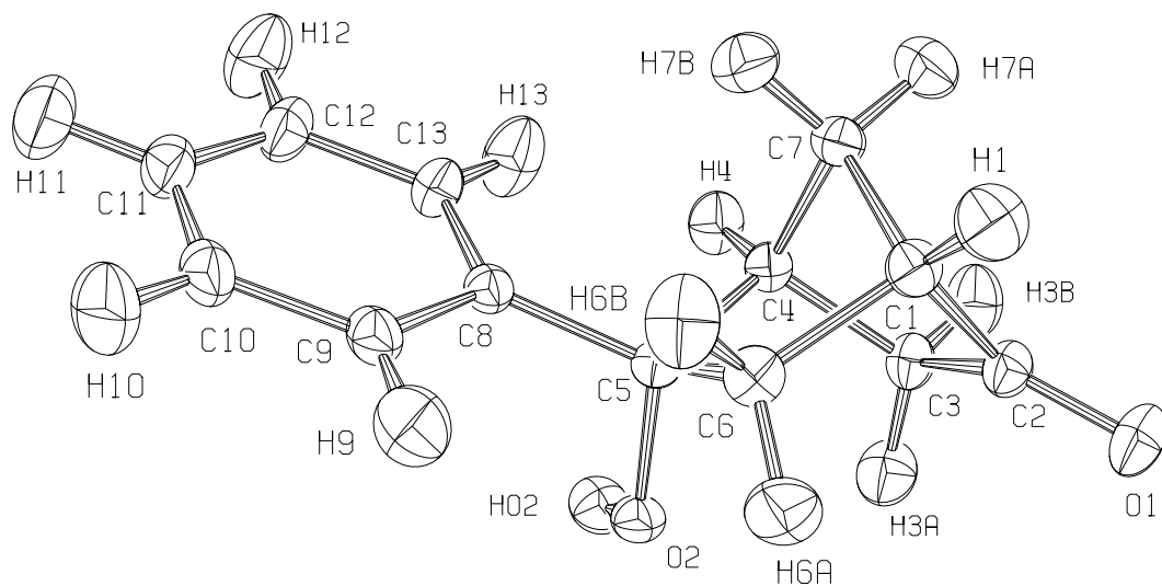
PHENYL-HYDROXYL-NORBORNANONE
