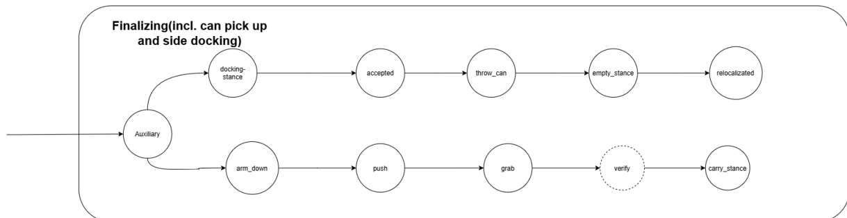
Figure 5: Conceptual finalization branches for can pickup and bin placement. The labels summarize physical stages; the implementation realizes bin placement through calibrated side docking, insertion, release, safe-home motion, and relocalization.
