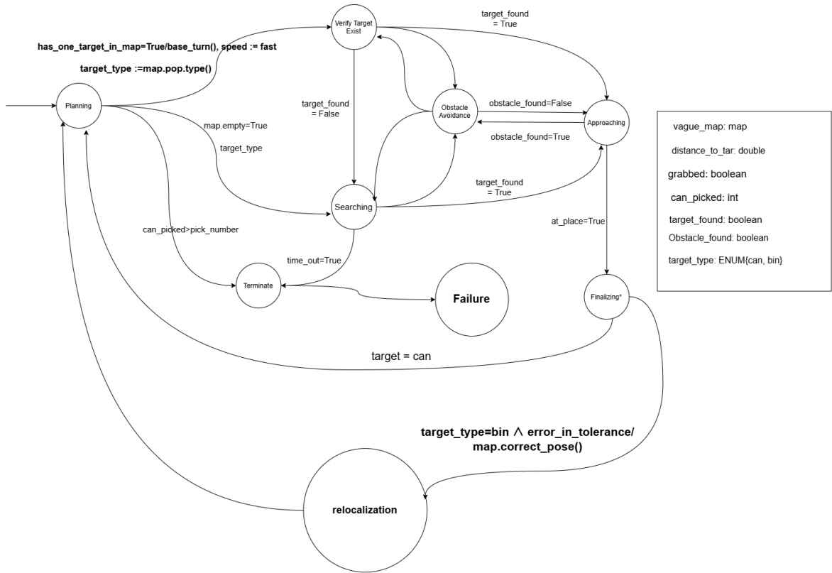
Figure 4: Simplified mission FSM showing planning, search, approach, avoidance, finalization, failure, and bin-based relocalization. It presents the control semantics rather than every production substate. Note that the syntax is semi-formal with some transitions omitted.
