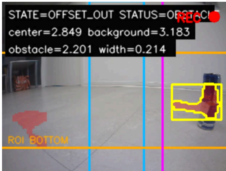
Figure 7: Recorded obstacle-debug HUD showing the collision corridor, extracted obstacle contour, selected side, tangent boundary, and relative-depth statistics.
