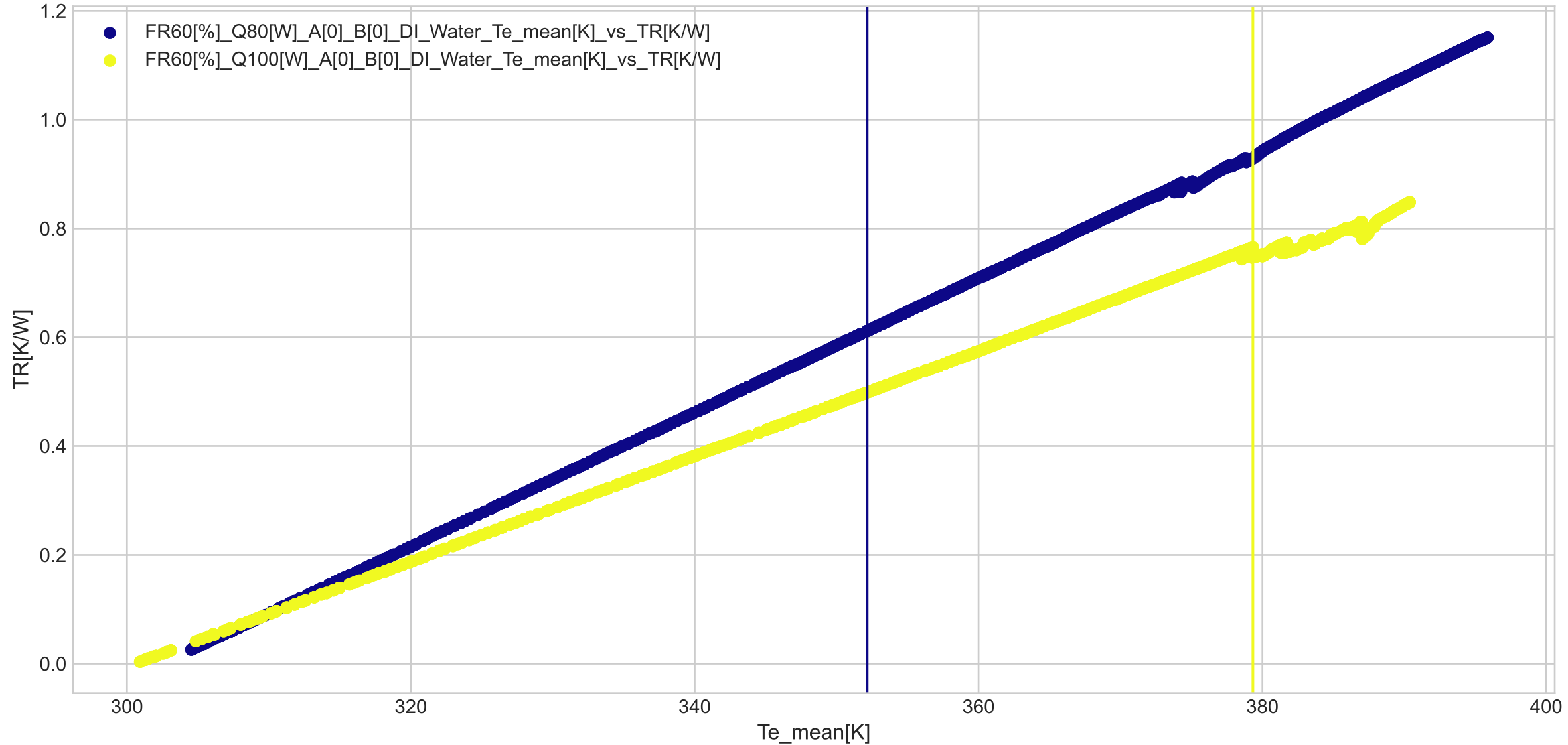
FR [60]% - Q [ 80 100]W - alpha [0] - beta [0] - DI_Water
