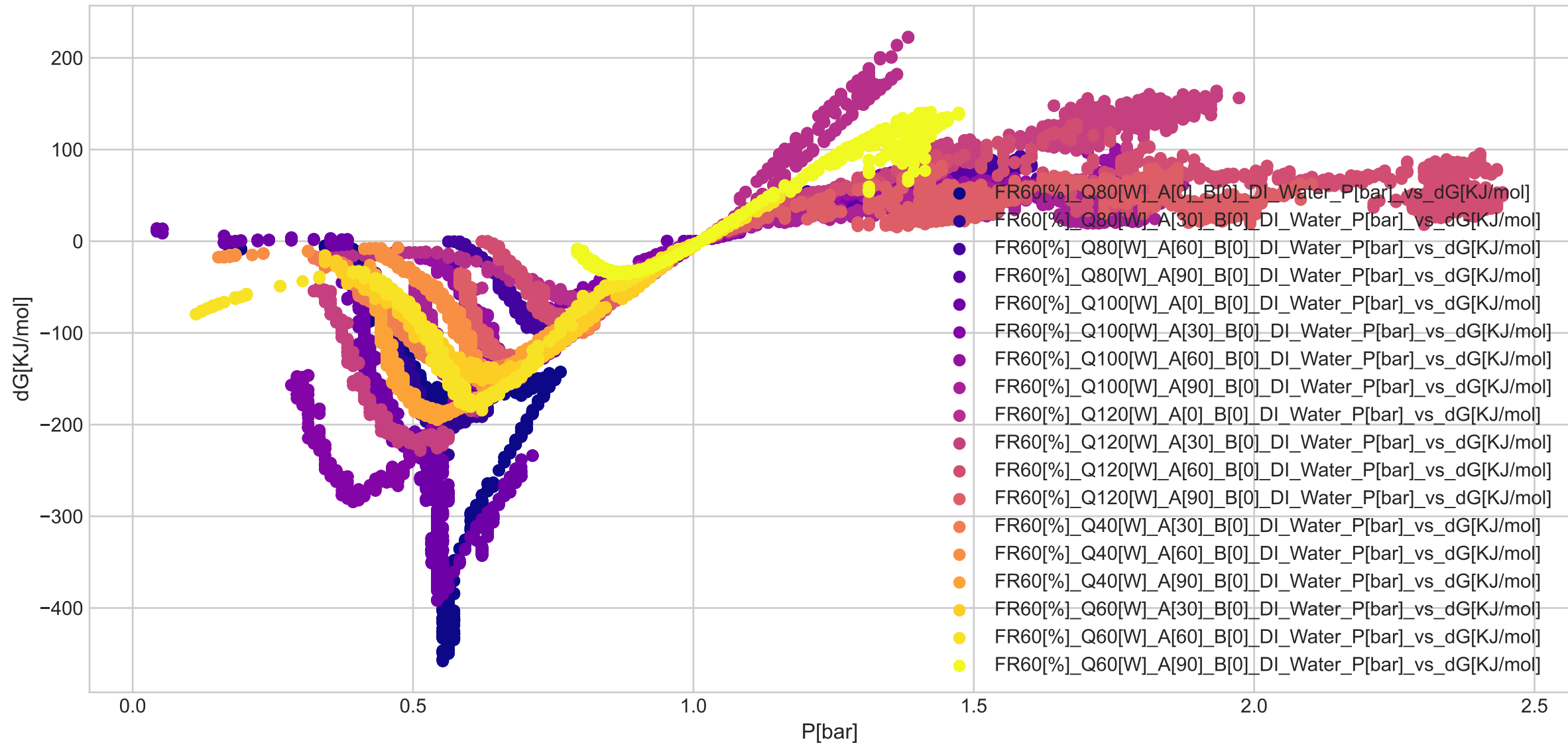
FR [60]% - Q [ 80 100 120 40 60]W - alpha [ 0 30 60 90] - beta [0] - DI_Water
