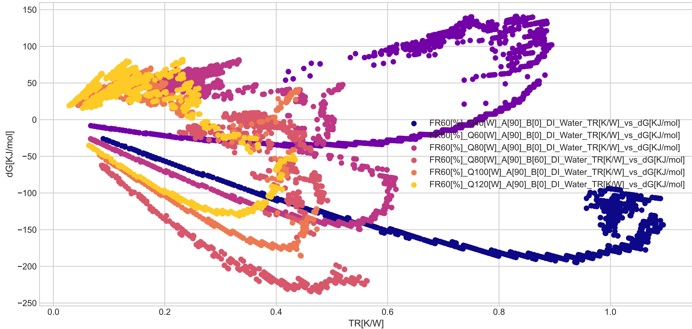
FR [60]% - Q [ 40 60 80 100 120]W - alpha [90] - beta [ 0 60] - DI_Water
