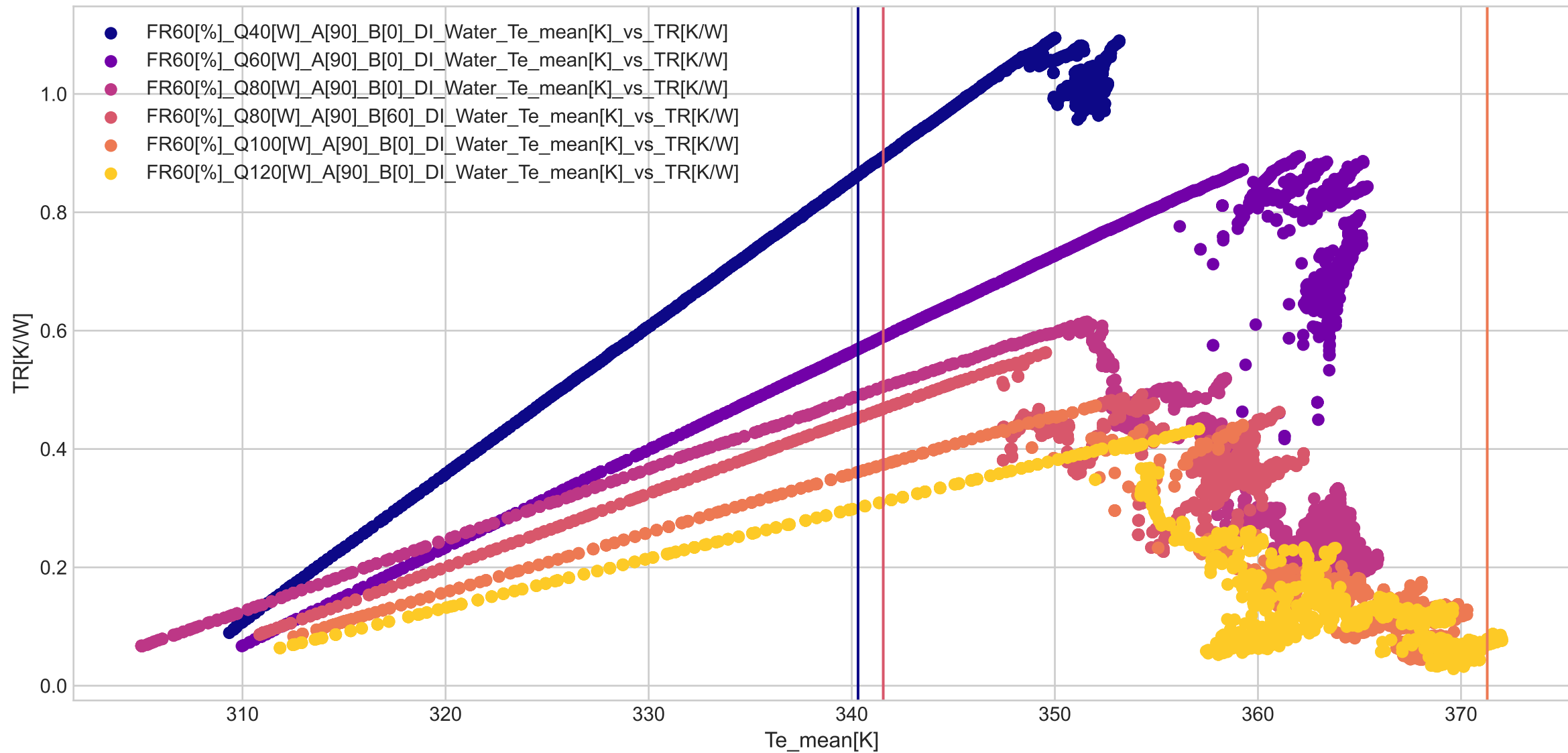
FR [60]% - Q [ 40 60 80 100 120]W - alpha [90] - beta [ 0 60] - DI_Water
