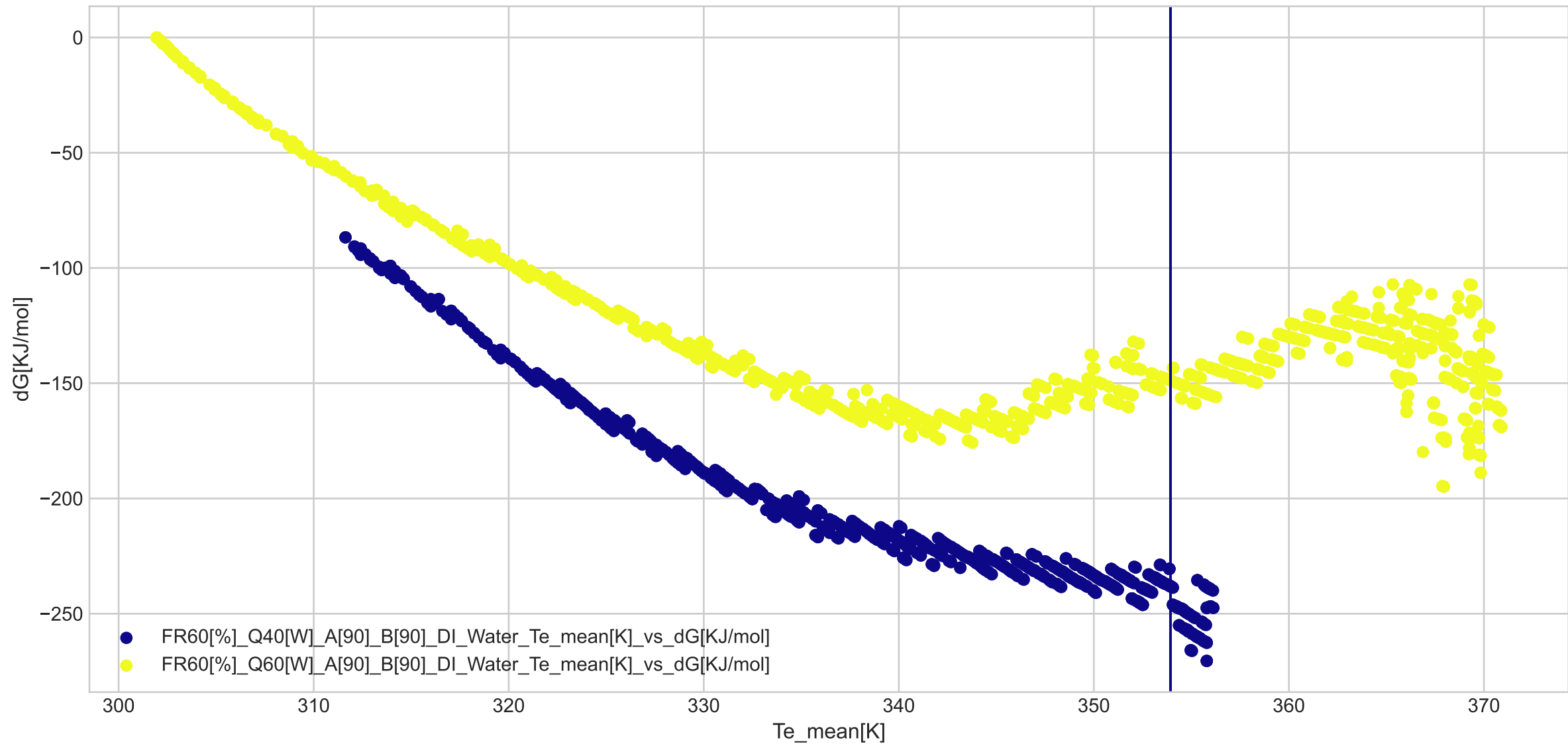
FR [60]% - Q [40 60]W - alpha [90] - beta [90] - DI_Water
