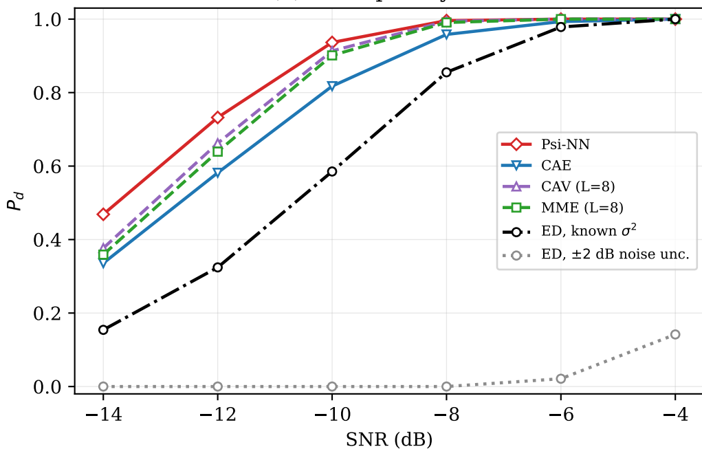
(b) 8 samples/symbol
