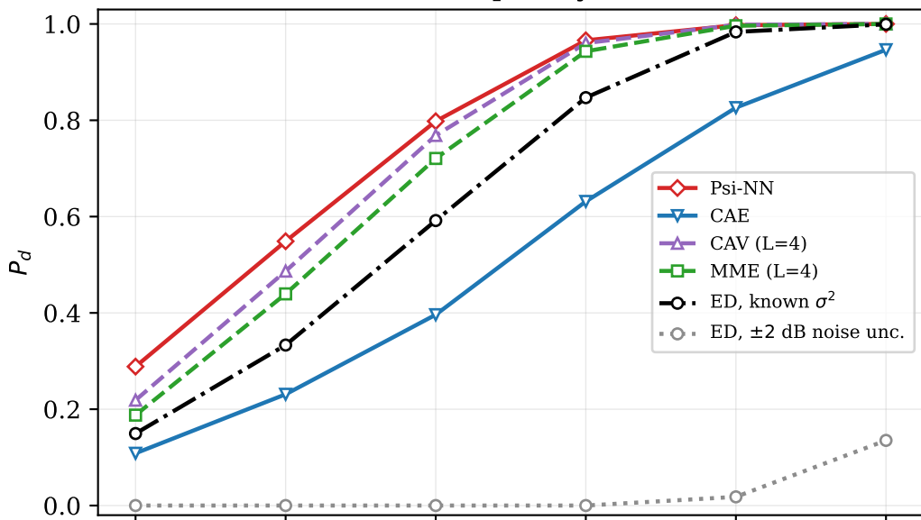
(b) 8 samples/symbol
