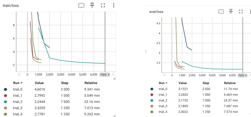
Development of train and validation losses of mT5 training across Optuna trials
