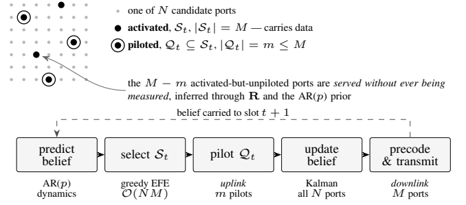
Fig. 1. Per-slot operation. The base station activates M of N candidate ports, but spends pilots on only m \leq M of them; the remaining M - m activated ports carry data while never being measured, their channels supplied by the belief alone. Both the activated set \mathcal{S}_t and the piloted subset \mathcal{Q}_t are chosen by minimizing the same expected free energy, which is what turns the pilot budget from a fixed cost into a design variable.
