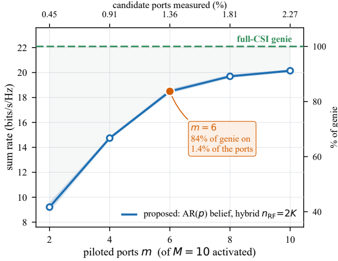
Fig. 2. Sum rate against the pilot budget m , at N = 441 ( 21 \times 21 ), M = 10 , K = 3 , n_{\text{RF}} = 6 , f_D T_s = 0.1 and 15 channel realizations; the band is the 95% confidence interval. The upper axis restates m as a fraction of the whole candidate grid: even when every activated port is piloted, the agent measures only 2.3% of the ports. Withdrawing pilots from ports that continue to carry data costs little down to m = 6 , below which the belief can no longer cover the gap.
