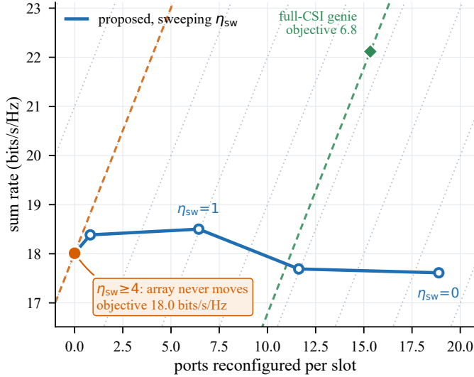
Fig. 3. Sum rate against reconfiguration cost as the switching weight \eta_{sw} is swept, at m = 6 over 8 realizations. Dotted lines are iso-objective contours of (6) at \eta_{sw} = 1 ; the two dashed contours pass through the genie and through our best operating point. The frontier is nearly flat — the agent moves from 18.9 reconfigured ports per slot down to none while the sum rate varies by 0.89 bits/s/Hz, and in fact peaks at \eta_{sw} = 1 rather than at \eta_{sw} = 0 : holding a port lets its belief sharpen, so some reluctance to move buys rate instead of costing it. The genie leads on raw rate but lies on a far worse contour, and is beaten on the objective for any \eta_{sw} > 0.27 .
