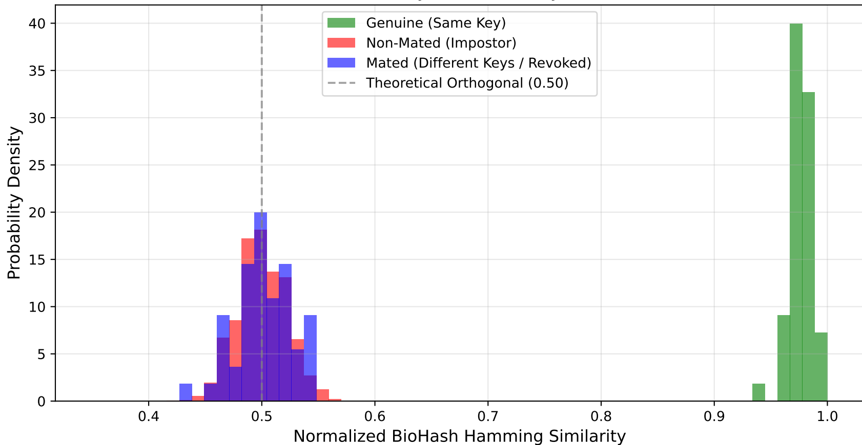
ISO/IEC 24745 Unlinkability & Revocability Score Distributions
