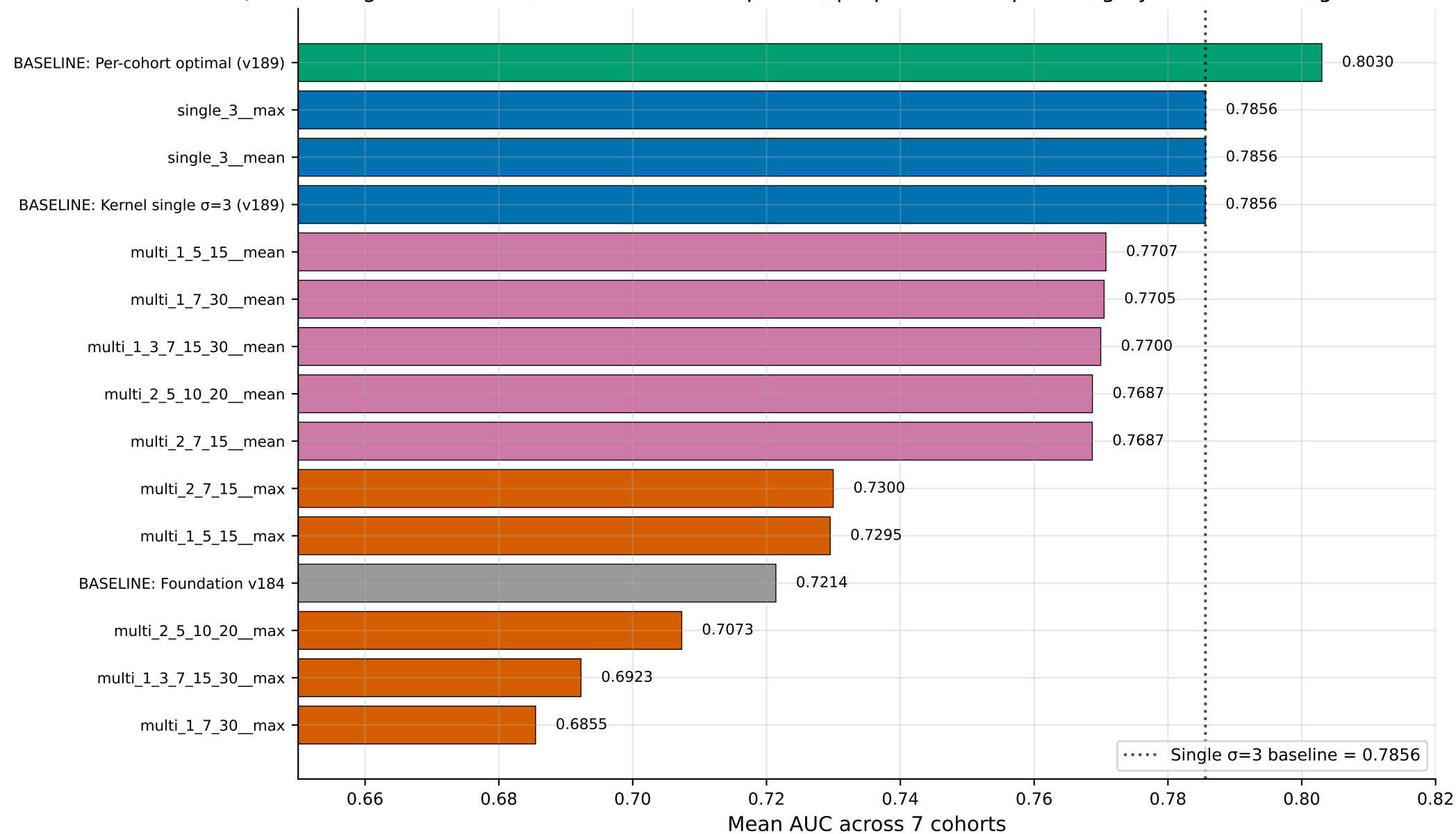
v191 multi-scale kernel ranking — single \sigma=3 BEATS all 10 multi-scale variants tested (blue = single \sigma=3 winner; vermillion = max-pooled; purple = mean-pooled; grey = foundation; green = oracle)
