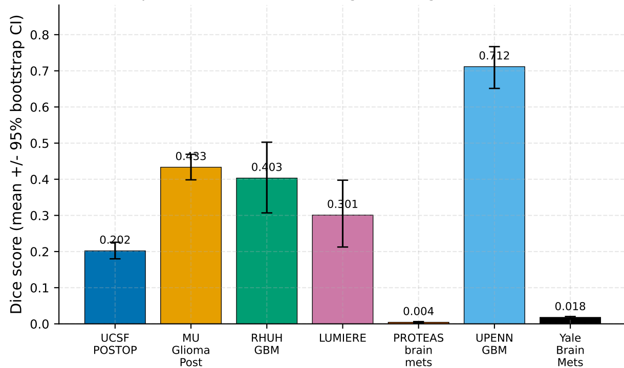
v184: Per-patient Dice score on outgrowth region (LOCO + zero-shot)
