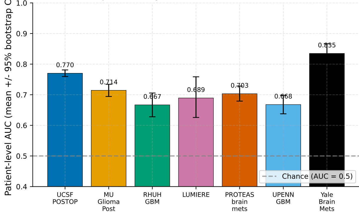
v184: Per-patient outgrowth-detection AUC across 7 cohorts
