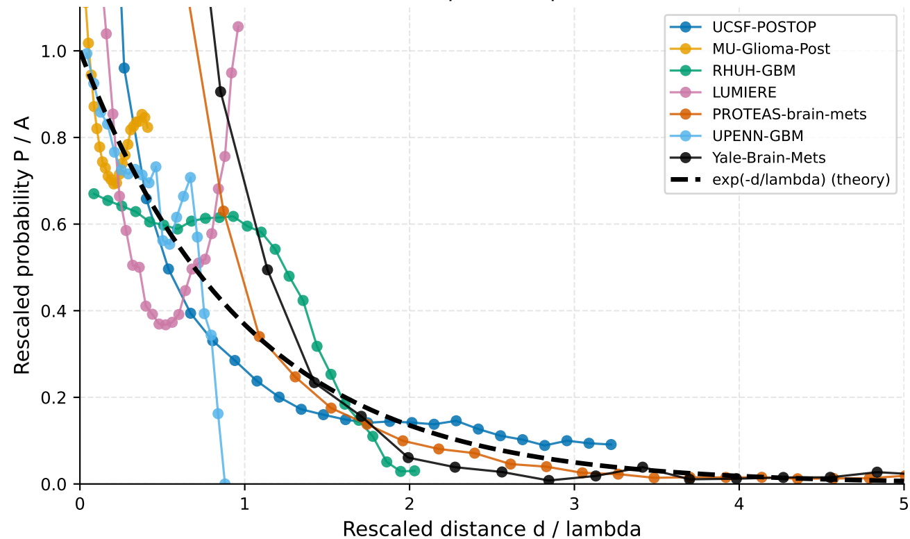
Linear: collapse to exp(-x) curve
