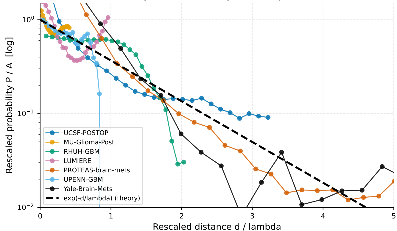
Log: should be straight line slope -1
