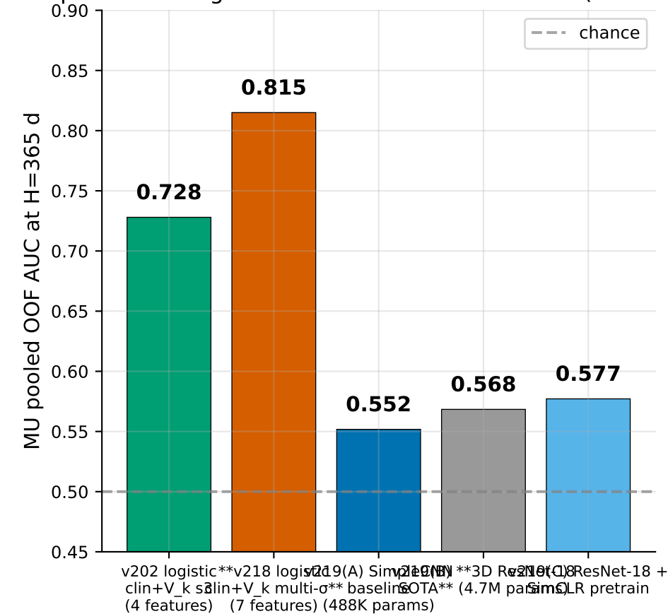
A. Logistic vs SOTA architectures Simple multi- \sigma logistic CRUSHES SOTA ResNet-18 (+0.247 AUC)
