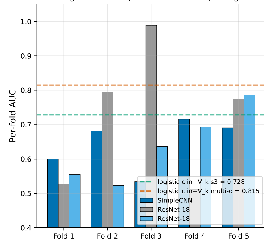
C. Per-fold AUC distribution ResNet-18 high variance (overfit at n=130): range 0.51-0.99
