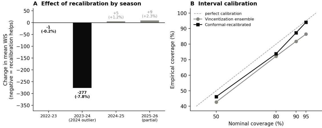
Figure 4: Effect of conformal recalibration on the dengue ensemble. (A) Change in mean WIS per season, conformal-recalibrated minus Vincentization ensemble, so negative means recalibration helps. The asymmetry is the point: a gain of 277 WIS units in the 2024 outlier season against costs of 5 and 9 units in the two ordinary seasons that follow it, roughly thirty to fifty times smaller. (B) Interval calibration: empirical versus nominal coverage. Recalibration moves the outer intervals (90, 95) toward the diagonal.
