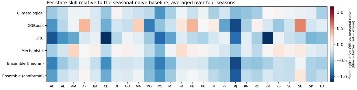
Figure 6: S6 Fig. Per-state skill relative to the seasonal-naïve baseline. Mean log relative WIS by model and state, averaged over the four seasons. Blue is better than baseline, red is worse, and the diverging scale is centred on baseline parity. A red-blue scale is used rather than red-green so that the comparison remains readable under red-green colour vision deficiency and in greyscale. The underlying values are released as log_relative_wis_by_state.csv for readers who need the numbers rather than the colours.
