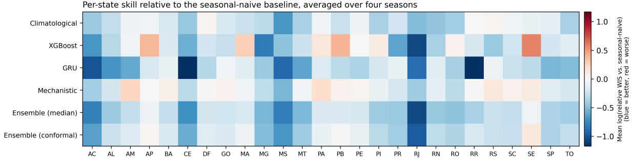
Figure 6: S6 Fig. Per-state skill relative to the seasonal-naive baseline. Mean log relative WIS by model and state, averaged over the four seasons. Blue is better than baseline, red is worse, and the diverging scale is centered on baseline parity. A red-blue scale is used rather than red-green so that the comparison remains readable under red-green color vision deficiency and in grayscale. The underlying values are released as log_relative_wis_by_state.csv for readers who need the numbers rather than the colors.
