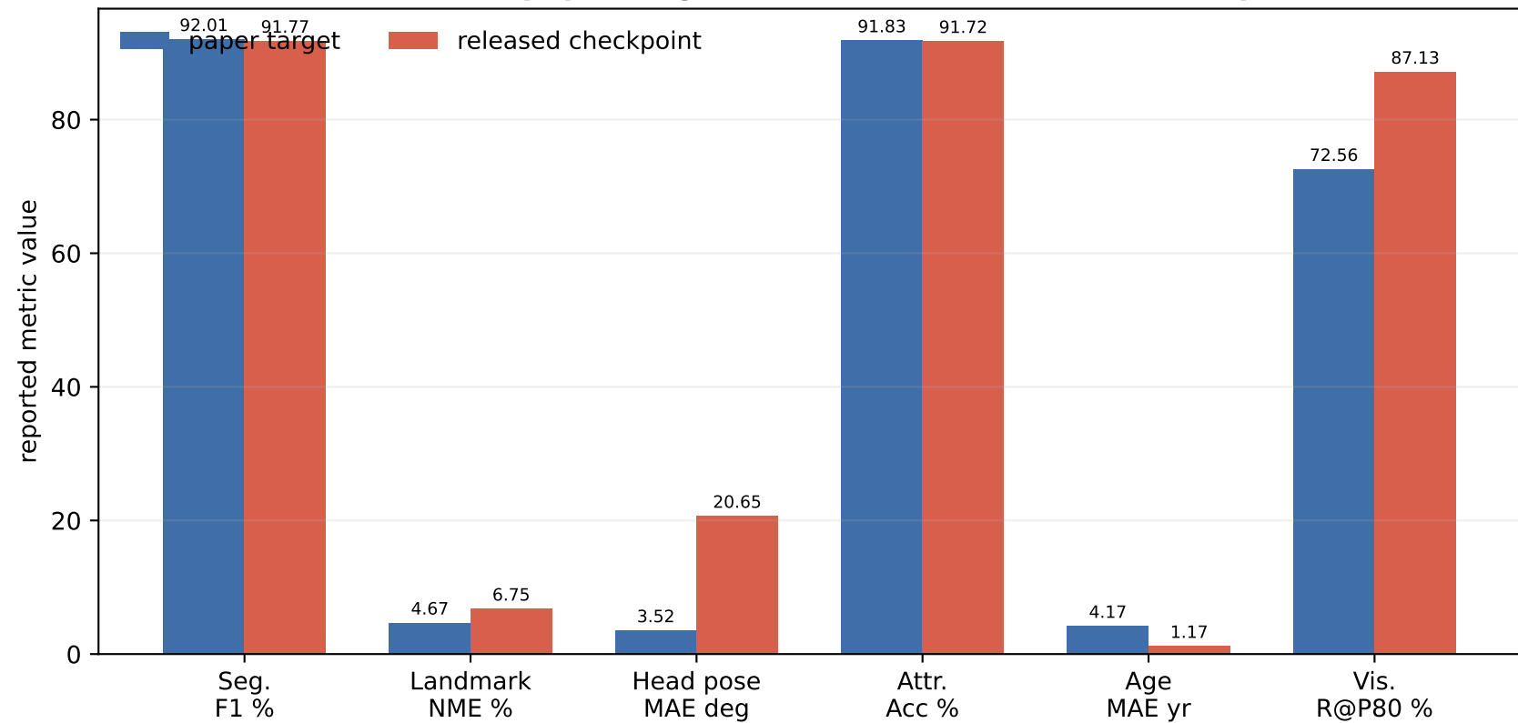
Baseline inference: paper target vs. normalized released-checkpoint value
