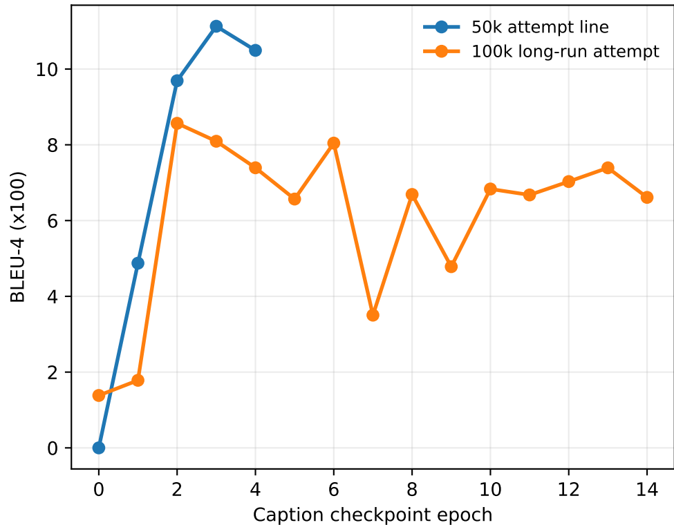
BLEU-4 vs Caption Epoch
