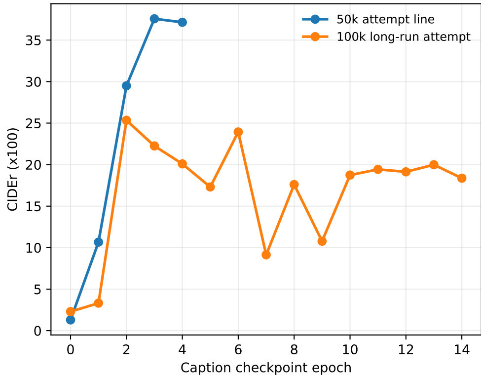
CIDEr vs Caption Epoch
