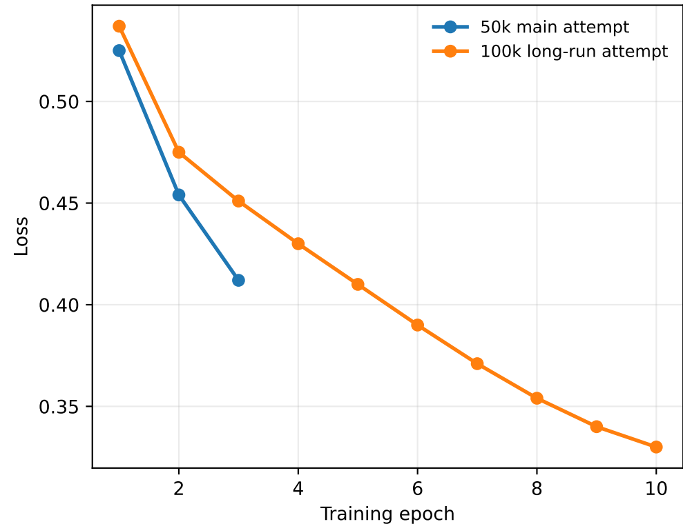
Stage 1 Train Loss
