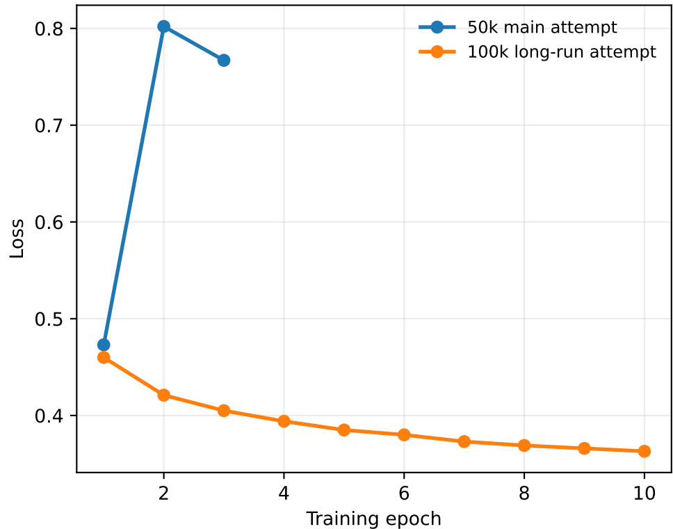
Stage 2 Train Loss
