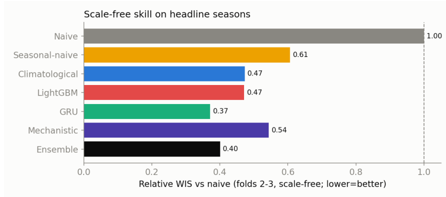
Figure 4: Metric-dependent rankings. Scale-free relative WIS on the ordinary seasons compared with magnitude-weighted mean WIS. The single-model ranking reorders: the deep network, weakest by mean WIS on the outlier, is strongest on ordinary seasons by the scale-free metric. Figure to be redrawn as an explicit rank-reordering (slope) chart with the current values.
