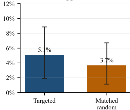
Disappearance
