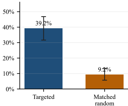
Answer change
