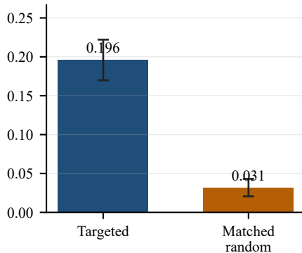
Centroid drift
